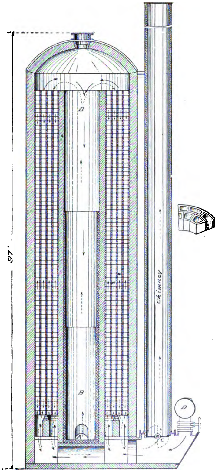
Fig. 95. Diagram of the J. Kennedy Variety of the Cowper Hot-blast Stove at Duquesne.
